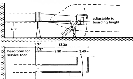
3 Swivel landing bridge
